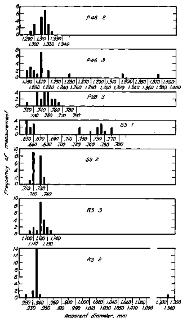
FIGURE 5. Effective diameter values of individual particles tested 20 times with the Mattson apparatus.
