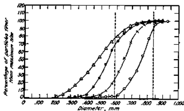
FIGURE 4. Particle-size distribution as determined by the Mattson apparatus of 20- to 30-mesh shot, Ottawa sand, river sand, and crushed limestone.
