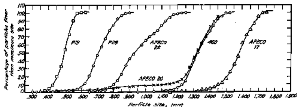
FIGURE 3. Percentage of particles of different samples of peening and cleaning shot finer than given sizes.
