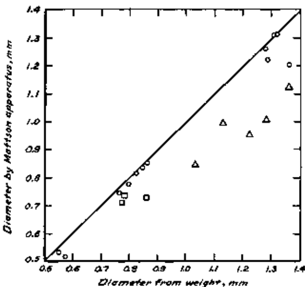
FIGURE 6. Relation of average diameter as determined by the Mattson apparatus to that determined from microweighings of individual particles.
